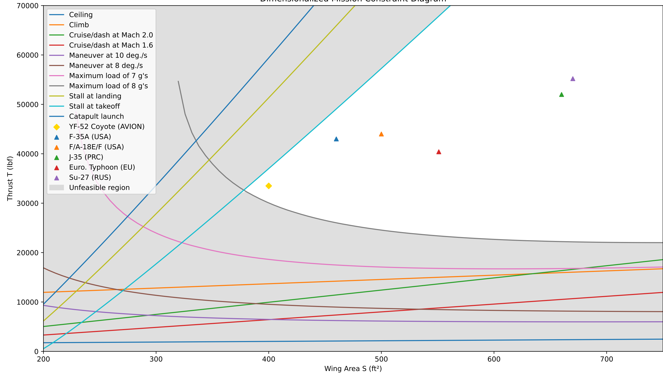
Dimensionalized Mission Constraint Diagram
